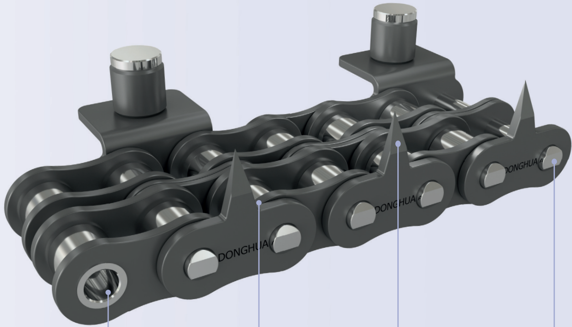
Hardened spikes
