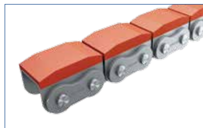
橡胶附板链 Roller chains with elastomer profile
