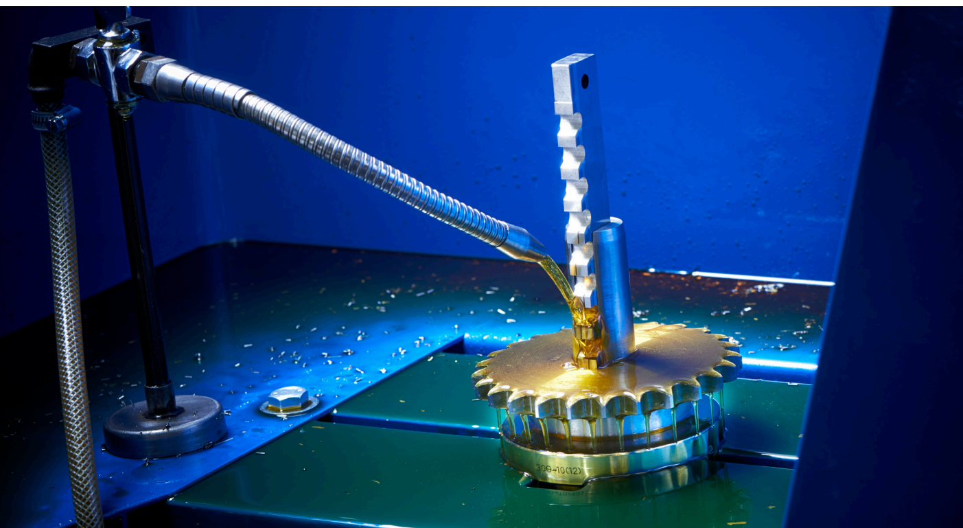
Precision keyway broaching
